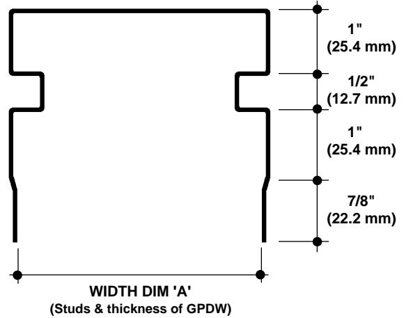
SWC-212R-2 (Shown) CUSTOM WALL CAP NO SCALE W/ 1/2" REVEAL
