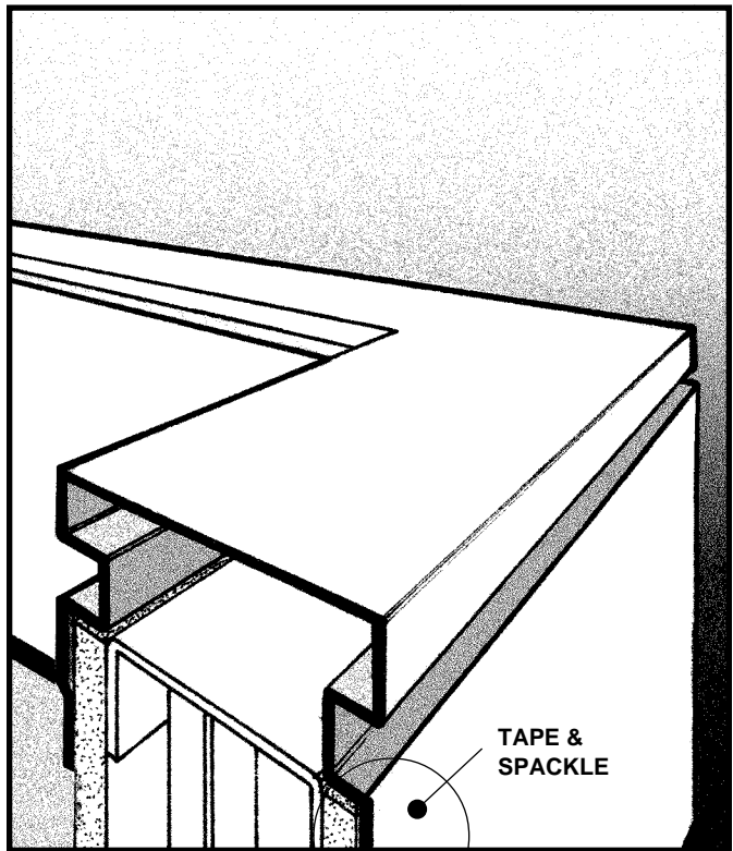
SWC-212R-2 (Shown) CUSTOM WALL CAP NO SCALE W/ 1/2" REVEAL
