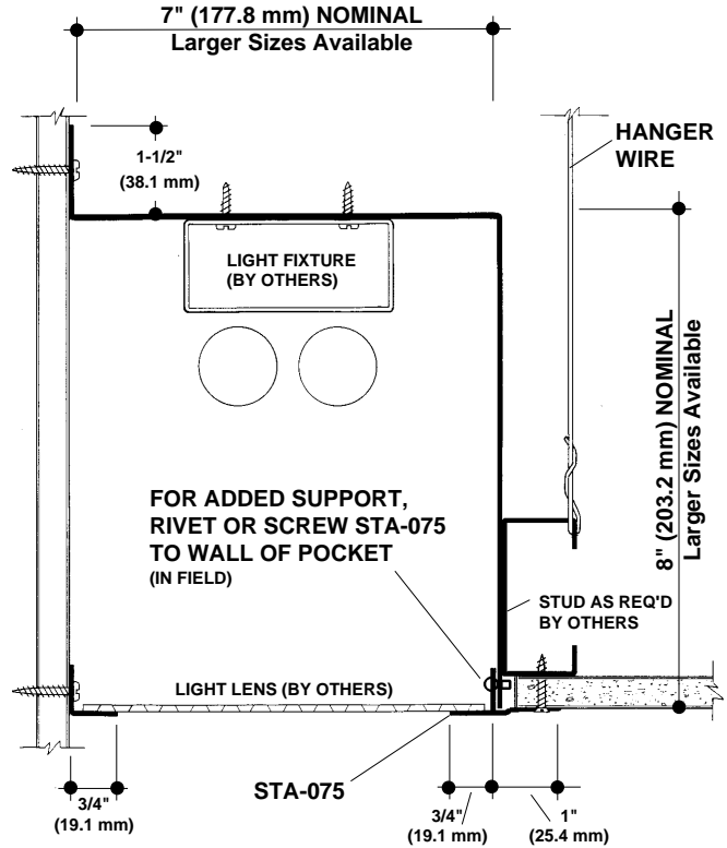
SLP-700-800 NO SCALE
