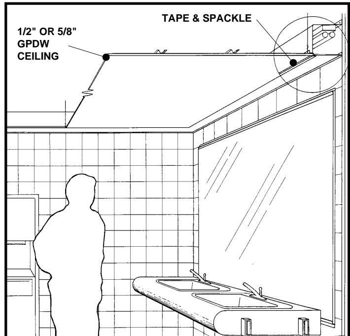
SLP-700-800 WITH GPDW TYPE CEILING NO SCALE
