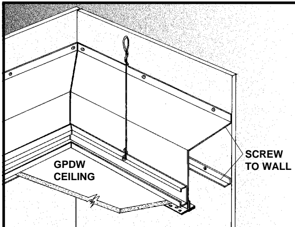
SLP-700-800 NO SCALE
