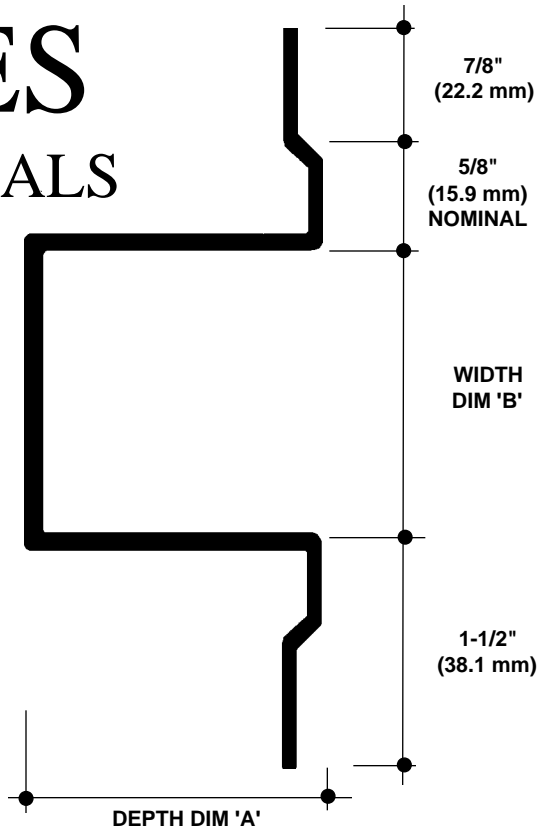
CUSTOM SWR-CD WALL REVEAL NO SCALE SECTION
