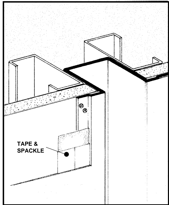
CUSTOM SWR-CD WALL REVEAL NO SCALE SECTION
