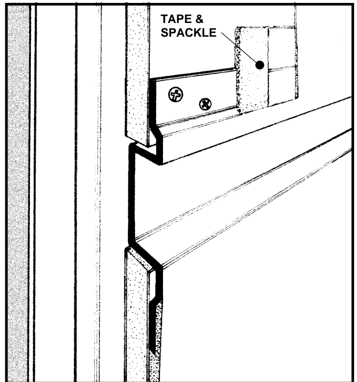
CUSTOM SWR-CW WALL REVEAL NO SCALE SECTION
