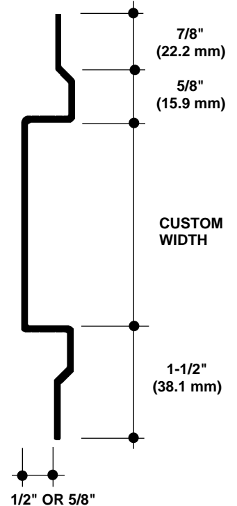
CUSTOM SWR-CW WALL REVEAL NO SCALE SECTION
