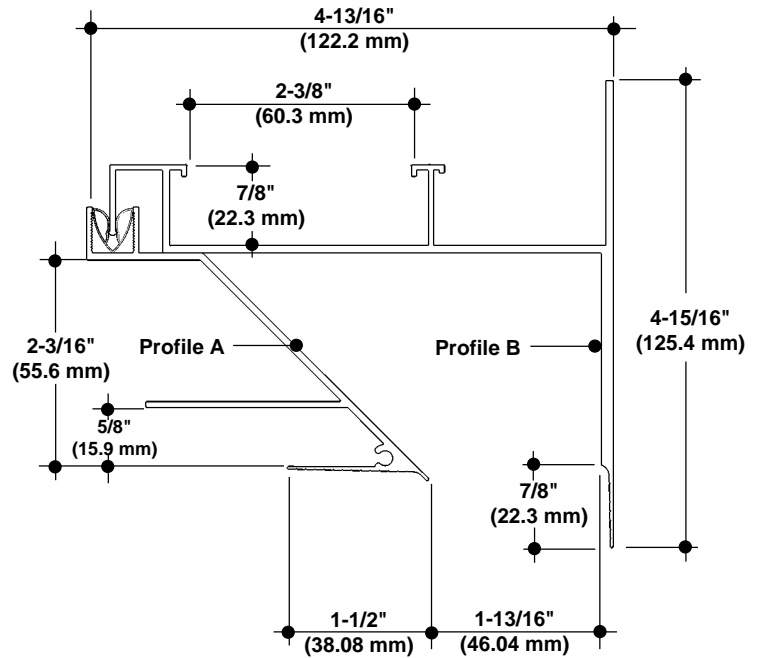
FCT-PF FLOATING CEILING TRIM NO SCALE SECTION
