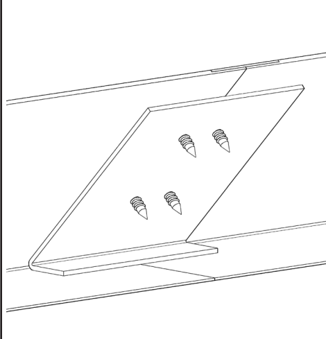
Backplate View
