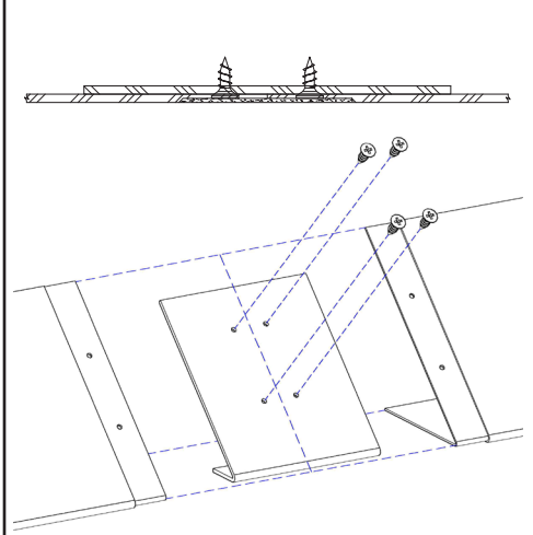
Joint Detail
