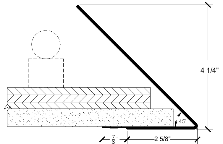
Connection Detail
